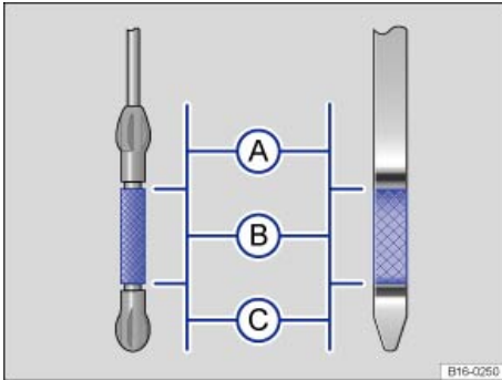
Fig. 156 Oil dipstick with engine oil level marks.
