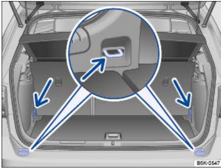
Fig. 94 In the luggage compartment: Tie-downs.
