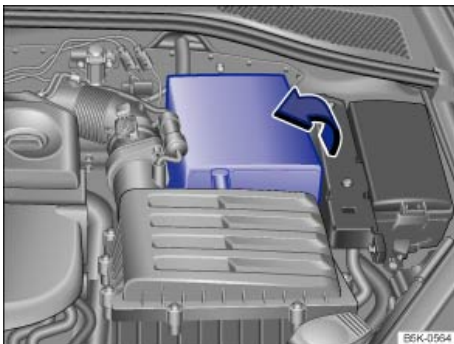
Fig. 161 In the engine compartment: Open the sleeve covering of the vehicle battery.
