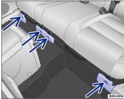
Fig. 100 Front attachment of the rear seat.
