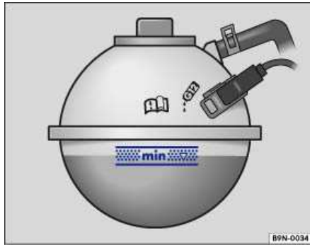
Fig. 172 Coolant expansion tank in the engine compartment.
