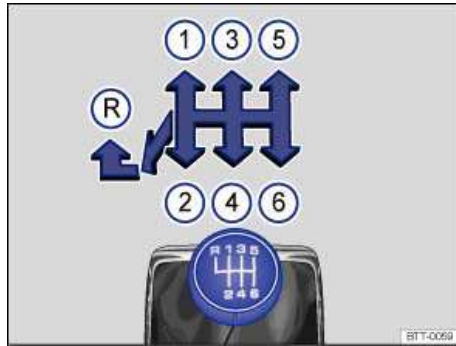
Fig. 140 Gearshift pattern of a 6-speed manual transmission.
