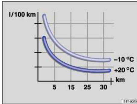
Fig. 148 Fuel consumption in l/100 km at 2 different outside air temperatures.
