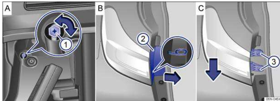
Fig. 209 In the side of the luggage compartment: Releasing the tail light, removing the trim panel and removing the screws.
