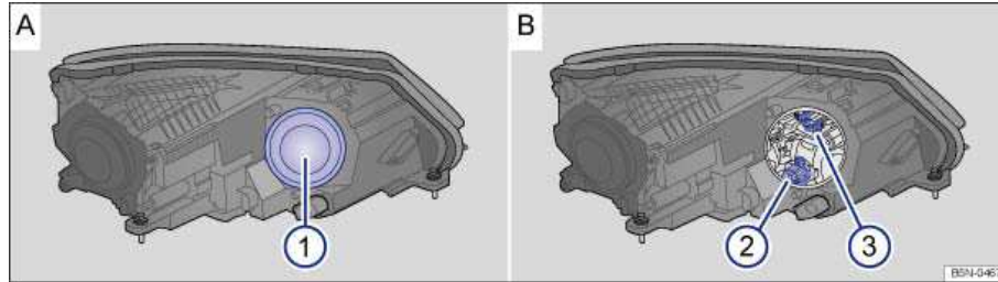
Fig. 205 In the engine compartment: Cover 1 on the left headlight for the turn signal bulb holder 2 and the cornering light bulb holder 3.
