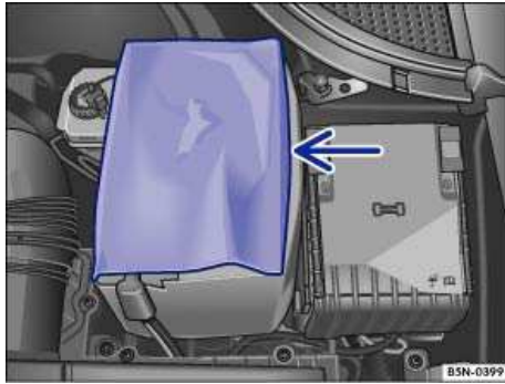
Fig. 175 In the engine compartment: Open the sleeve covering of the vehicle battery.
