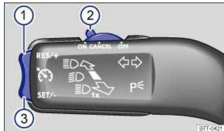
Fig. 150 On the left side of the steering column: Cruise control buttons and switches.
