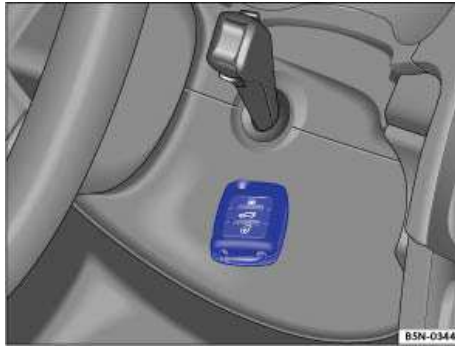
Fig. 137 Emergency starting feature on vehicles with Keyless Access.
