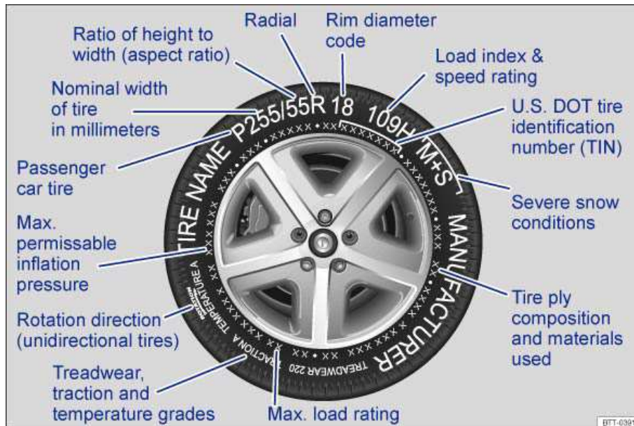
Fig. 118 International tire labeling.
