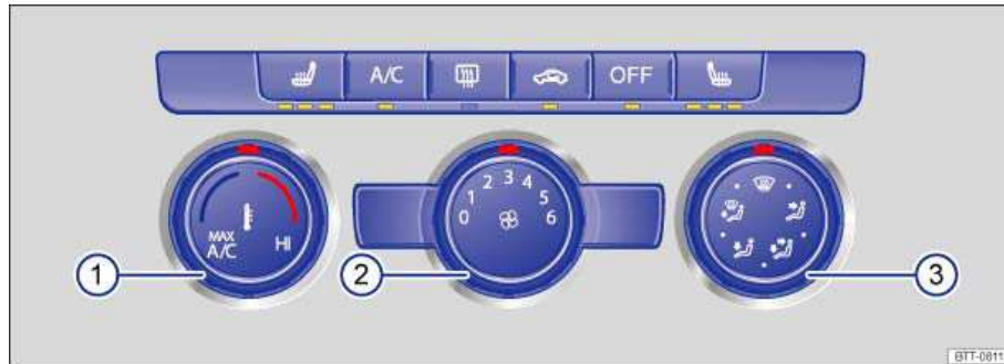
Fig. 158 In the center console: Manual AC controls.
