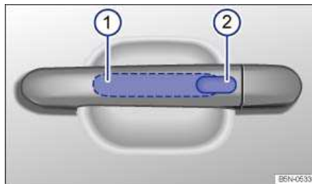
Fig. 30 Keyless Access with push button start: Sensor 1 for unlocking on the inside of the front door handles. Sensor for locking 2 on the outside of the door handles.
