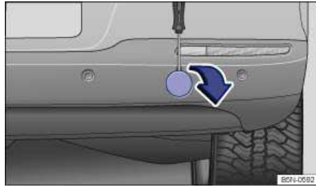
Fig. 214 On the right in the rear bumper: Cover.
