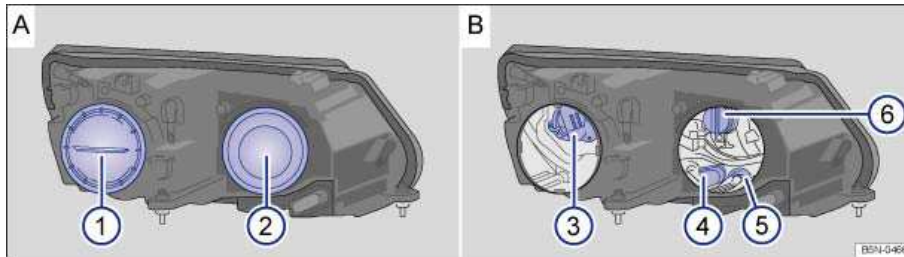
Fig. 204 In the engine compartment: Cover 1 on the left headlight for the low beam bulb holder 3 and cover 2 for the parking light bulb holder 4, turn signal bulb holder 5 and high beam or daytime running light bulb 6.
