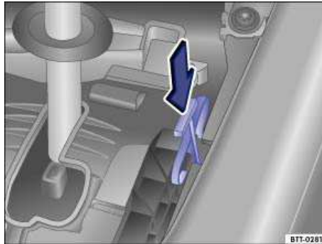
Fig. 187 Releasing the selector lever lock.
