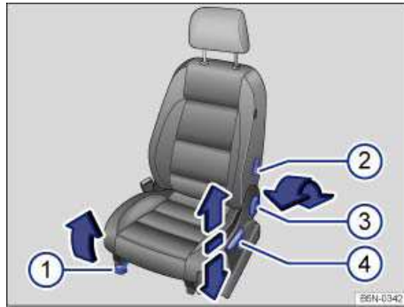
Fig. 41 Controls on the driver seat.
