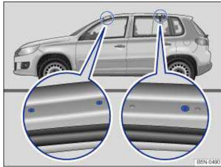
Fig. 109 Vehicles without roof railing: Attachment points for the base carrier and roof rack.
