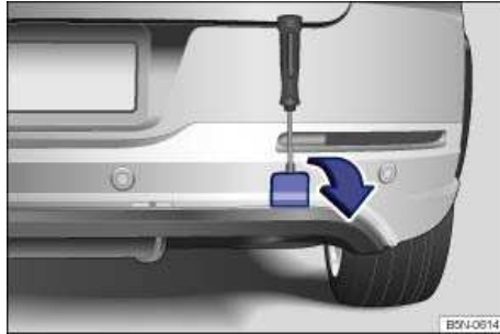
Fig. 216 On the right rear bumper: Removing the cover.
