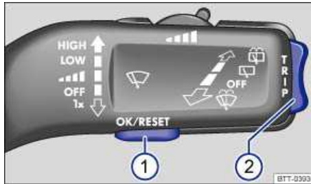
Fig. 18 Premium version (vehicles without menu control multi-function steering wheel): Control buttons 1 and 2 on the windshield wiper lever.
