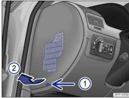
Fig. 345 On the left side of the instrument panel: Remove the fuse box cover.
