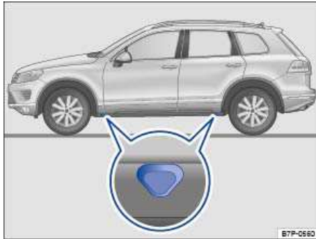
Fig. 338 Lift points for the jack.
