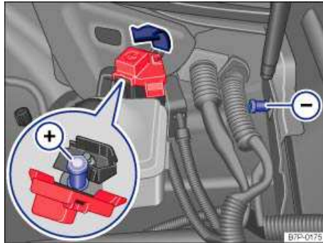
Fig. 349 In the engine compartment: Positive jump-start terminal + and negative jump-start terminal -.
