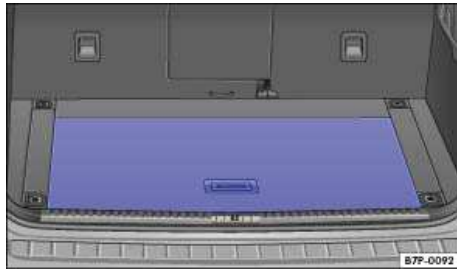
Fig. 261 Location of the high-voltage battery: under the luggage compartment floor.
